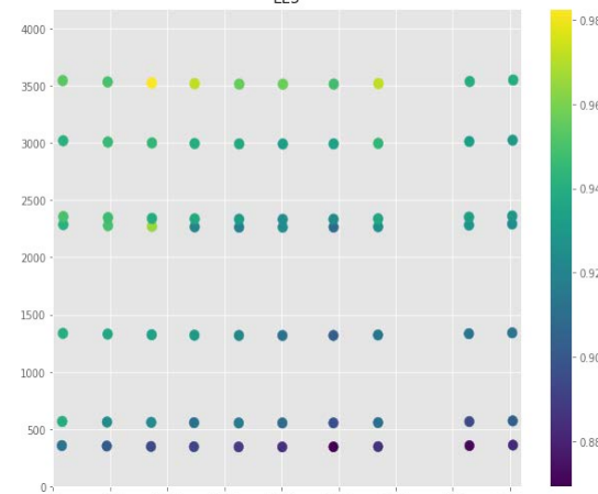
SM1 Subaru m1 Expls 2595 2596 argon neon doBckTrue best 85.7% of peak have a EE5 > 0.9
