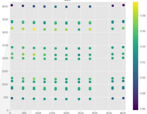
SM1 Subaru r1 Expls 2605 2606 argon neon doBckTrue best 93.3% of peak have a EE5 > 0.9
