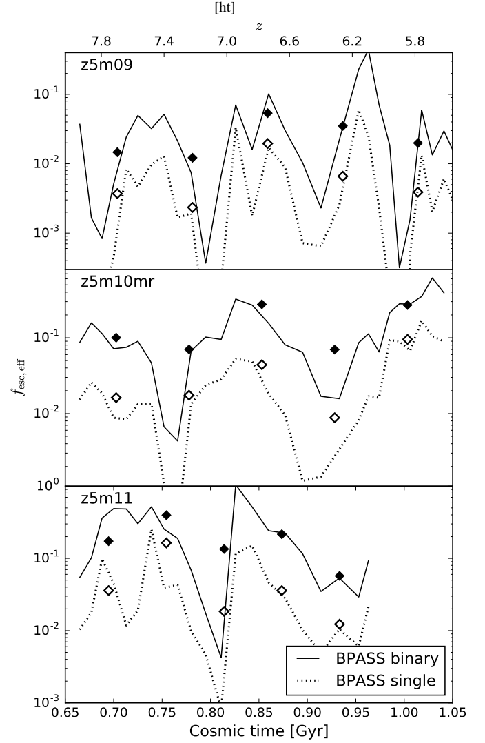
Figure 3. Effective escape fraction as a function time for z5m09, z5m10mr, and z5m11. In all cases, binary stellar models boost f_{\text{esc,eff}} by factors of \sim 4 –10. In more massive galaxies, the mean f_{\text{esc,eff}} reaches \sim 20\% , sufficient for reionization.
