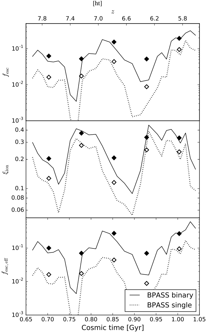
Figure 2. Top: True ionizing photon escape fraction f_{\text{esc}} , in our z5m10mr simulation (a \sim 10^{10} M_{\odot} halo at z = 6 ) as a function of redshift (or cosmic time). Lines show the instantaneous values in each snapshot, symbols are time-averaged in 100 Myr intervals. Middle: \xi_{\text{ion}} (as Fig. 1) as a function of time. Bottom: Effective escape fraction, f_{\text{esc,eff}} (Equation 2) as a function of time. In the single-star model, f_{\text{esc}} \lesssim 5\% most of the time, insufficient for reionization. Accounting for binary effects boosts \xi_{\text{ion}} by a factor \sim 1.5 – useful but insufficient to explain reionization. But it also boosts f_{\text{esc}} by factors \sim 3 –6 because the ionizing photons produced later (after t \gtrsim 3 Myr) preferentially escape, so the “effective escape fraction” f_{\text{esc,eff}} is increased by factors \sim 4 –10 and reaches the \sim 20\% values needed to explain reionization.
