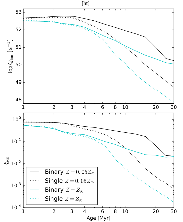
Figure 1. Top: Ionizing photon production rate, Q_{\text{ion}} as a function of age for a 10^6 M_{\odot} star cluster, predicted by different stellar evolution models. Bottom: Ratio of ionizing luminosity to 1500 \text{ \AA} luminosity, \xi_{\text{ion}} as a function of age for the same star cluster. We show both single-star models (dotted) and binary models (solid) at metallicities Z = 0.05 Z_{\odot} (black) and Z = Z_{\odot} (cyan), respectively. Including binaries leads to more massive stars at late times (from mass transfer and mergers), which dramatically enhances the ionizing photon production after t \sim 3 Myr. Q_{\text{ion}} also depends strongly on metallicity, with many more ionizing photons produced at low metallicity. STARBURST99 models, which also ignore binaries, are nearly identical to the BPASS single-star models at both metallicities.
