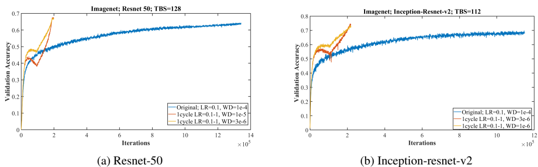
Figure 16: Training resnet and inception architectures on the imagenet dataset with the standard learning rate policy (blue curve) versus a 1cycle policy that displays super-convergence. Illustrates that deep neural networks can be trained much faster (20 versus 100 epochs) than by using the standard training methods.
