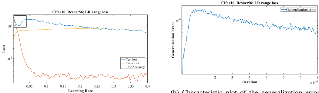
(a) Characteristic plot of training loss, validation accuracy, and validation loss.
