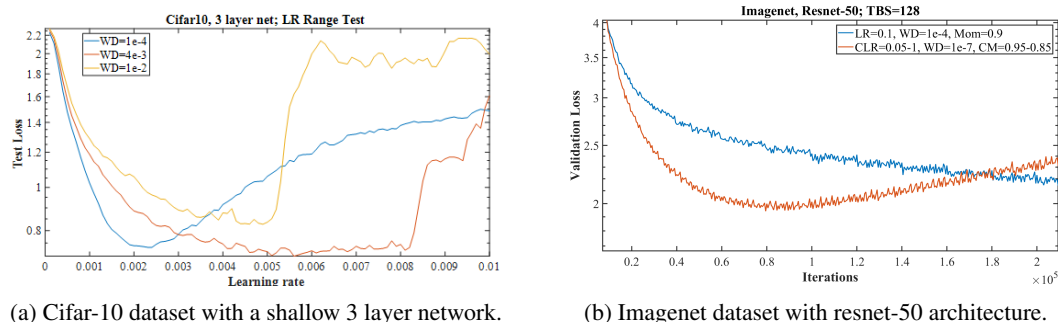
(a) Cifar-10 dataset with a shallow 3 layer network.
